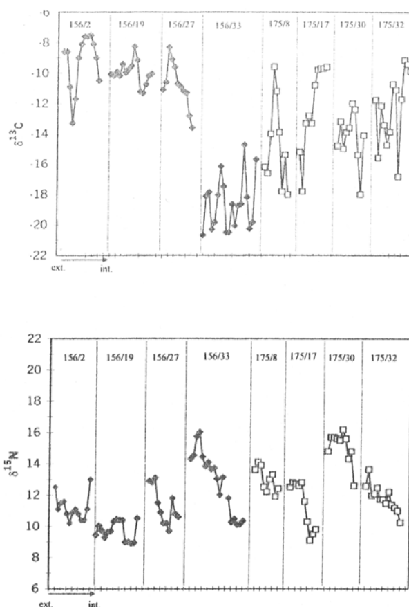
Fig.2 - The \delta^{13}\text{C} (A) and the \delta^{15}\text{N} (B) values of keratin horn samples from tomb 156 (diamonds) and tomb 175 (open square) analysed along the growth direction.
